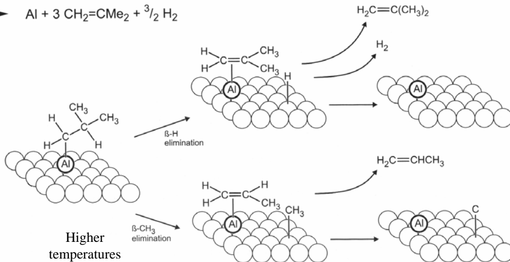
Figure 3-16. Schematic representation of the thermal decomposition of \text{Al}^i\text{Bu}_3 . The upper pathway (at low temperatures) results in the clean deposition. At higher temperatures (lower pathway) carbon impurities may be incorporated into the film.
