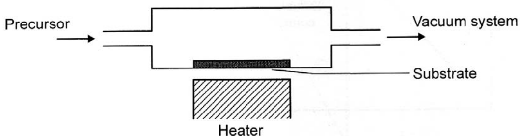
Figure 3-8. Schematic drawing of a cold-wall reactor.
