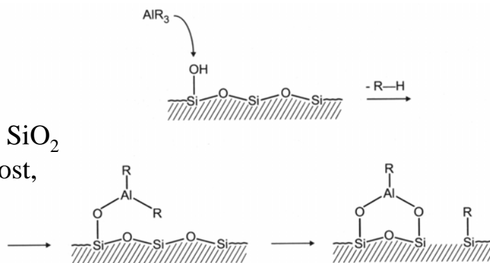
Figure 3-17. Inhibition of Al deposition from \text{AlR}_3 on a silica surface.
