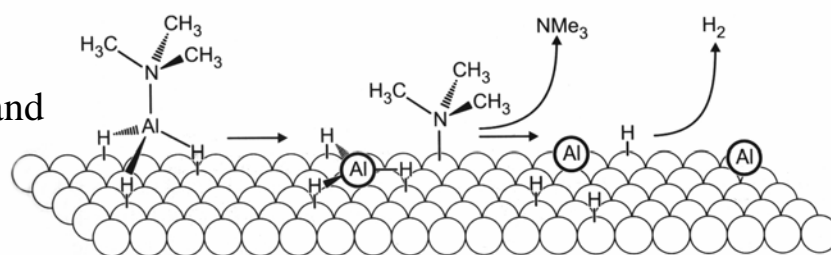
Figure 3-18. Thermal decomposition mechanism of \text{Me}_3\text{N}-\text{AlH}_3 on Al surfaces.
